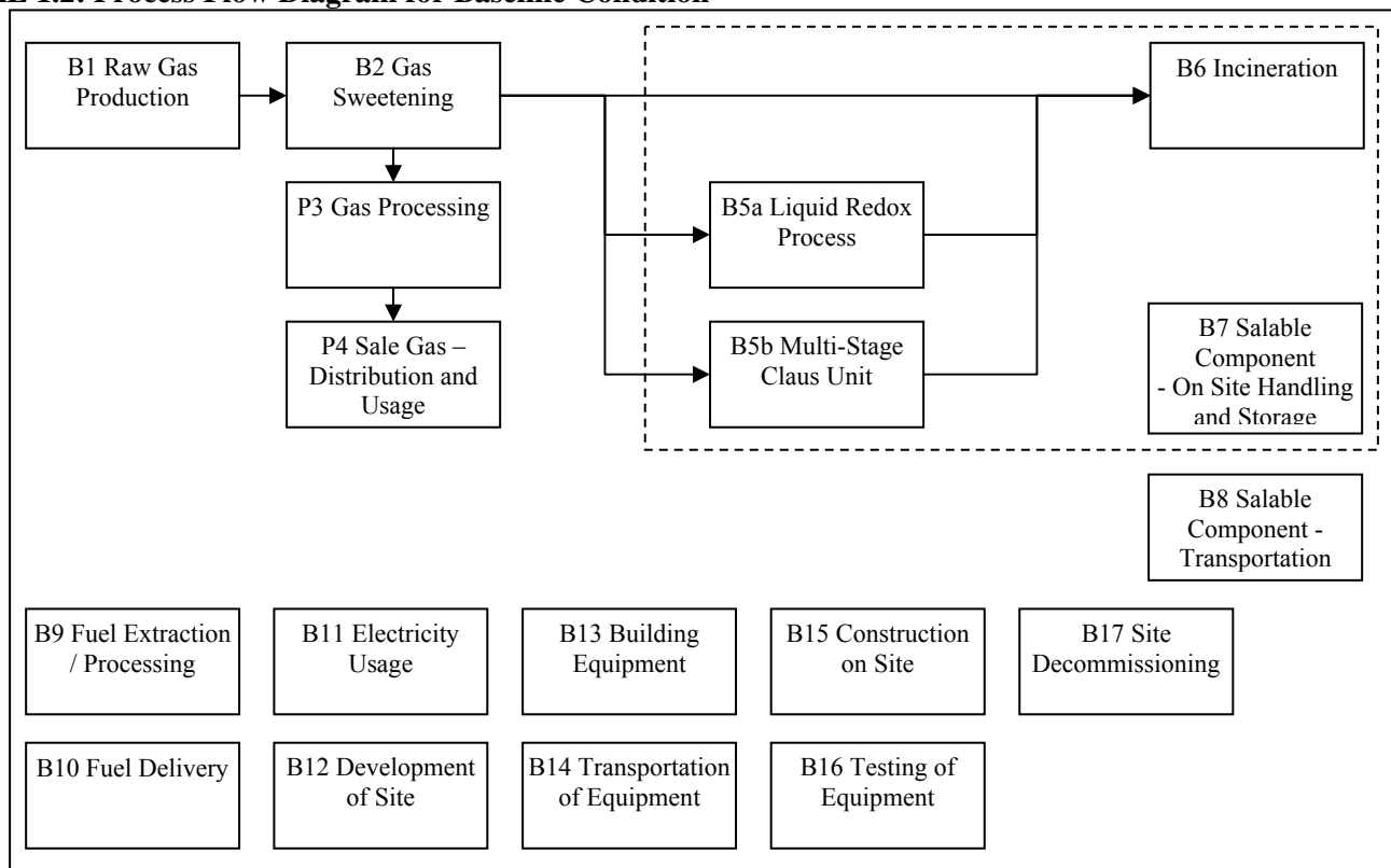
FIGURE 1.2: Process Flow Diagram for Baseline Condition
