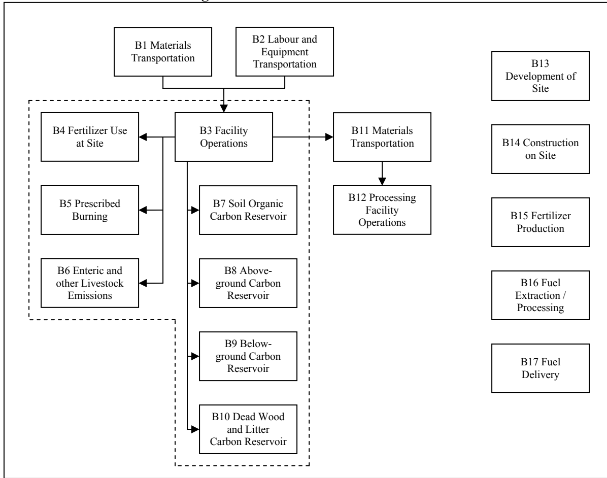
FIGURE 1.2: Process Flow Diagram for Baseline Condition
