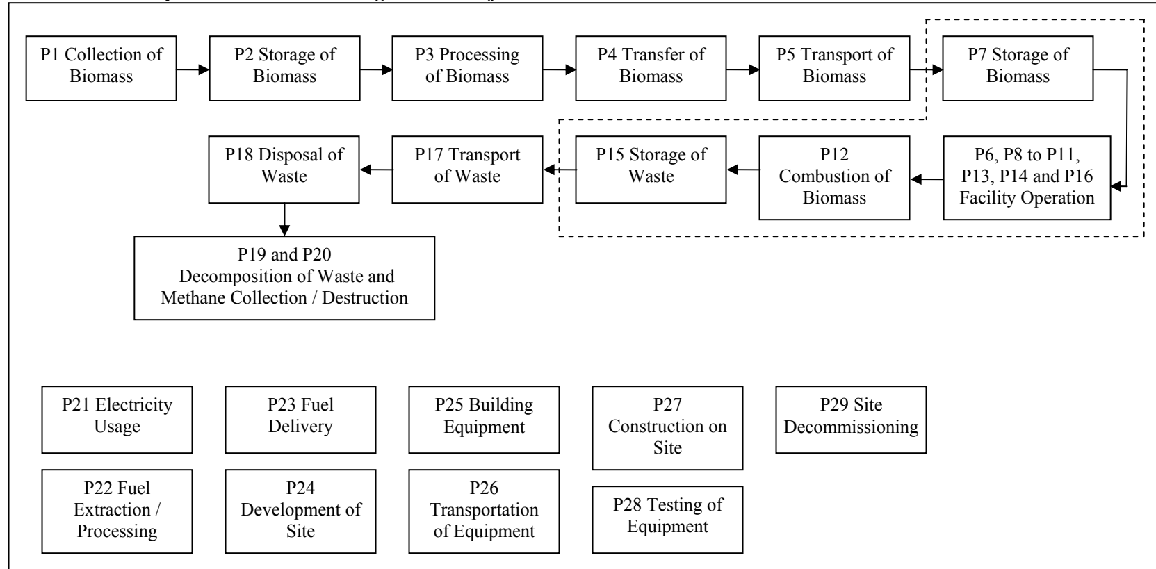
FIGURE 1.3: Simplified Process Flow Diagram for Project Condition
